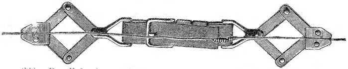
268. Parallel wire stretchers in operation, the slack being pulled up by the strap.
